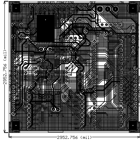
Drill Drawing.
