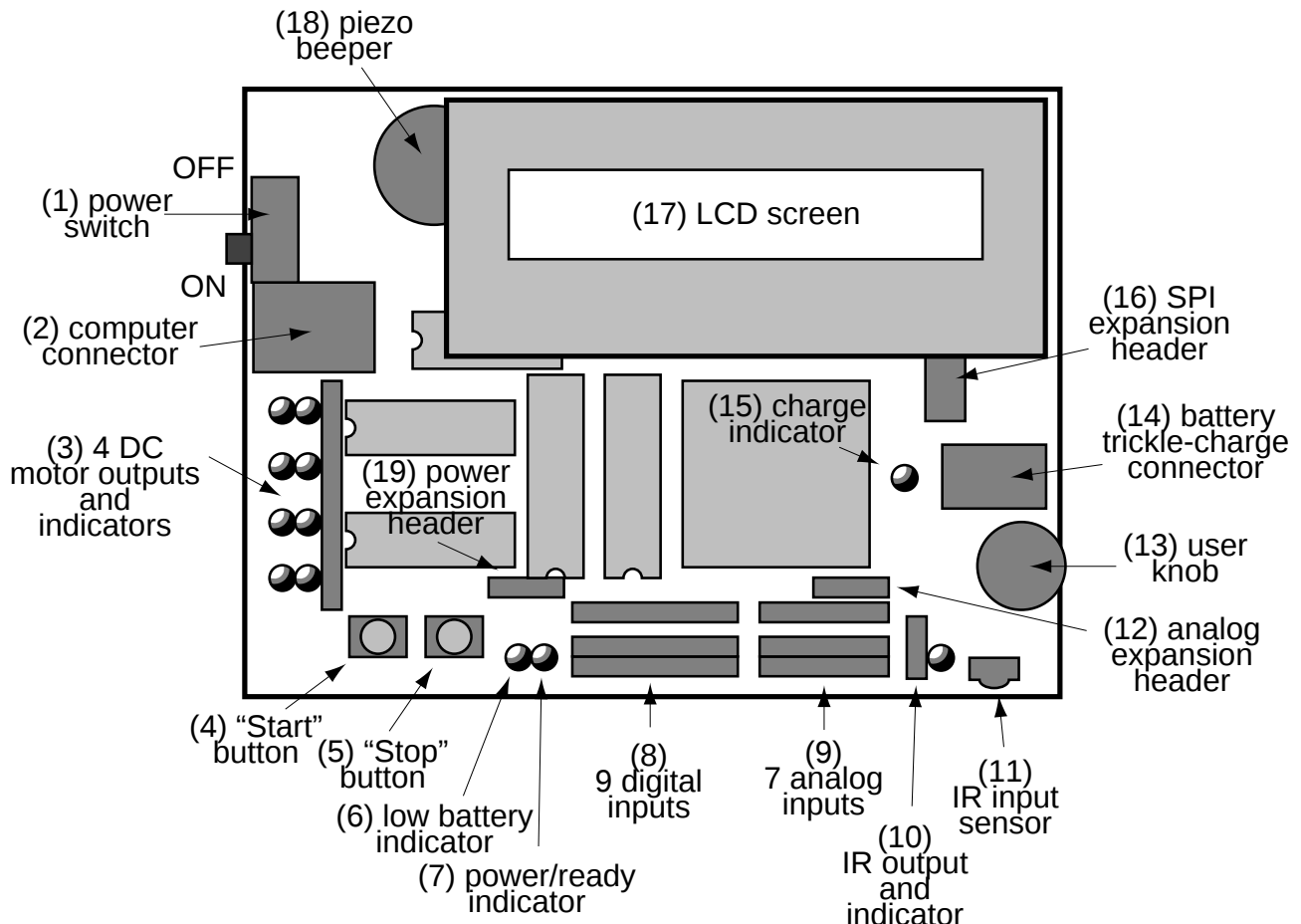
Figure 1: Labelled Handy Board Diagram
